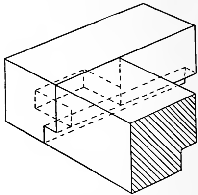
FIG. 442. JOINT FOR RABBETED FRAME.
